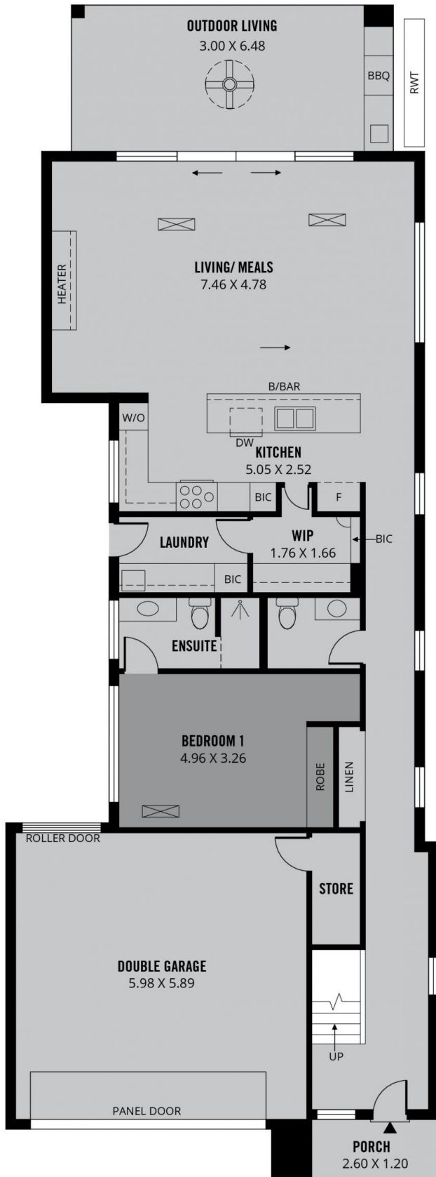
LOWER LEVEL
