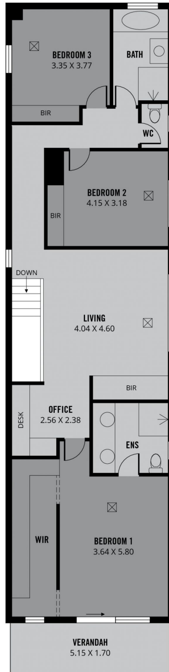
UPPER FLOOR
