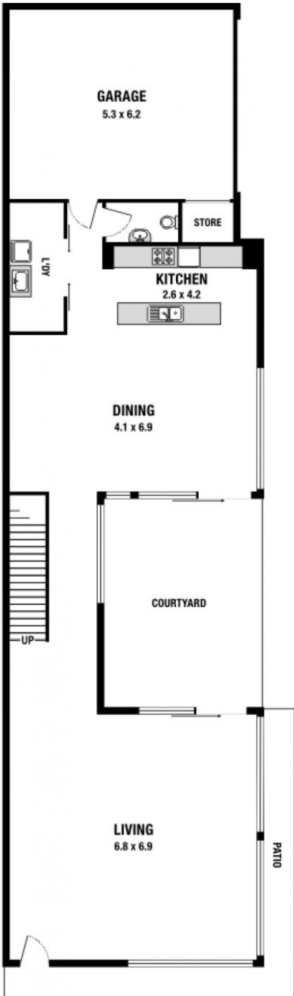
GROUND FLOOR
