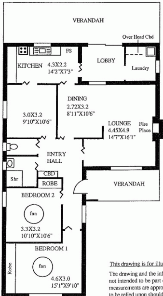
FLOOR PLAN
